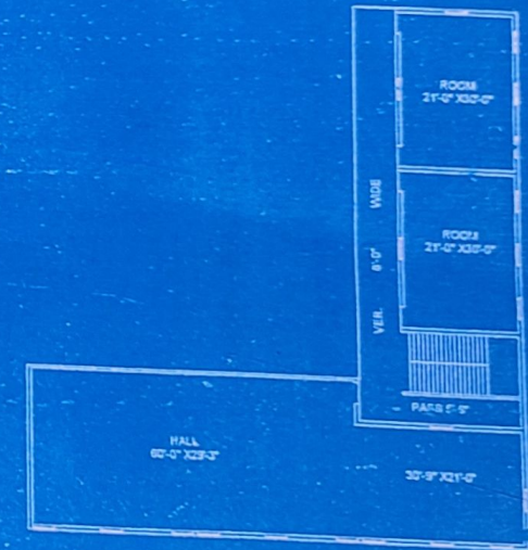
EX FIRST FLOOR
